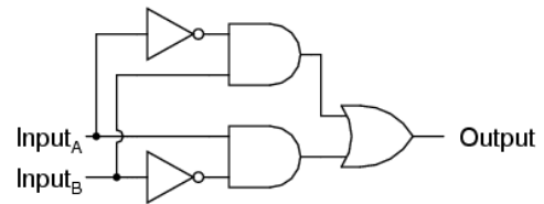
Exclusive-OR equivalent circuit
