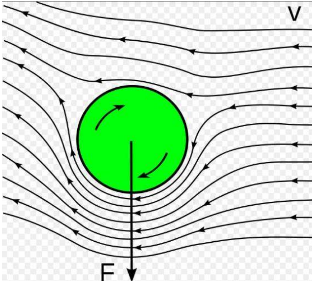
Magnus Effect lift
