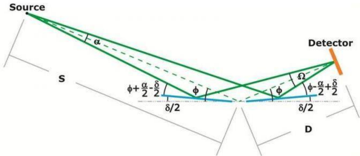
Lloyd's Mirror
