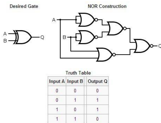
Exclusive OR (XOR)
