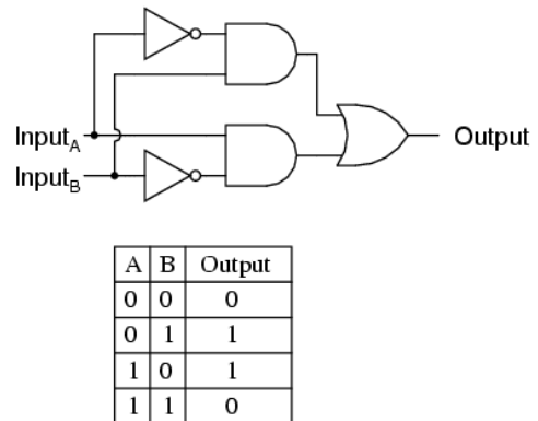
Exclusive-OR equivalent circuit
